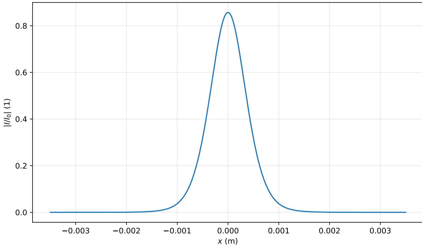
Intensity profile I(x, y = 0, z = 2.309m)/I_0 , P_{in}=0.6P_{cr} , artificial time
